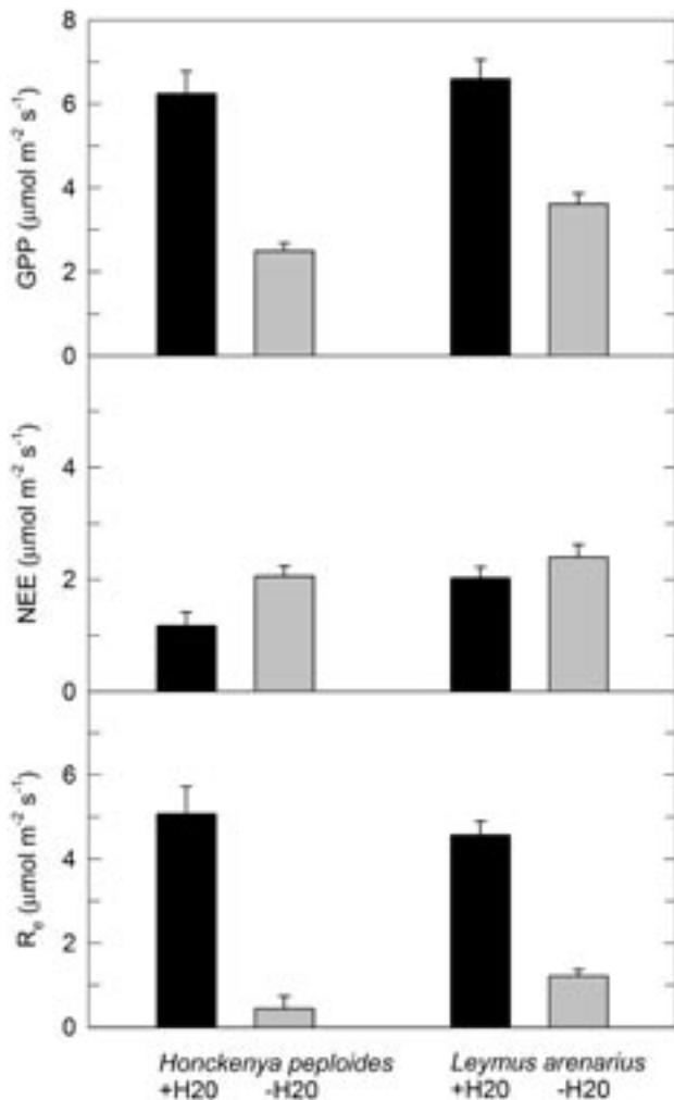
Figure 2. Gross photosynthesis (GPP), net ecosystem exchange (NEE) and ecosystem respiration ( R_e ) in a moist area (+H 2 O) and dry area (-H 2 O) on Surtsey in July 2006. Means and SE of 3–5 measurements per site.
