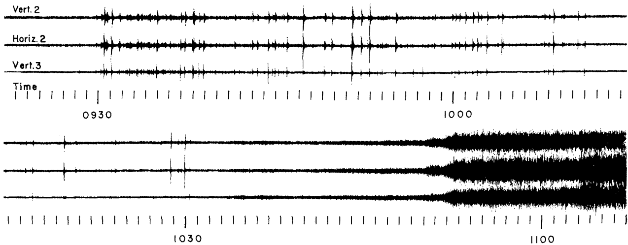
Fig. 5. The seismograms of August 19, 1966 showing the seismic activity associated with the beginning of a lava eruption on Surtsey. Shown are the seismograms of the vertical and one horizontal component of the northernmost seismic station and a vertical component of the southernmost station which was situated about 400 m from the fissure where the eruption broke out. The time is GMT.
